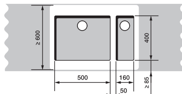
SUBLINE 500-U SUBLINE 160-U
